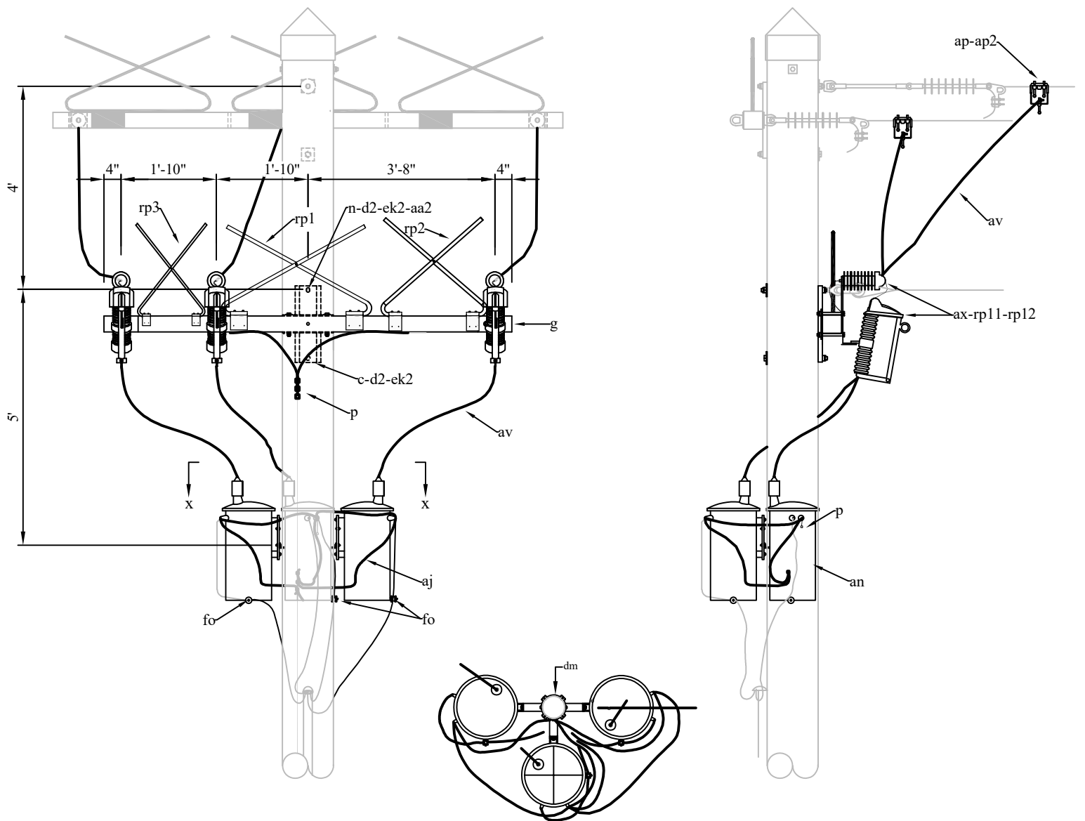
SECTION X-X
